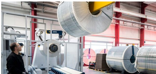
Machine operator Martin Müller heaves a 16-ton aluminum coil into the loading zone of the TRUMPF TruLaser 8000 Coil Edition.
