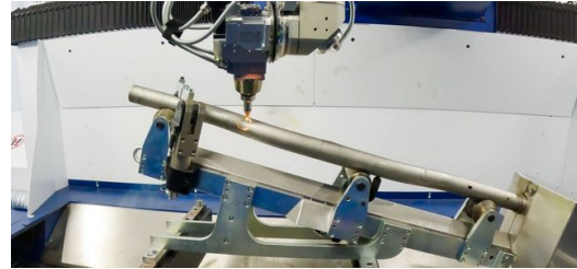
TRUMPF TruLaser Cell 8030 3D
