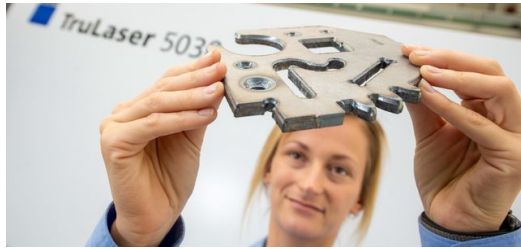
<p><span lang="EN-US">A worker checks a component she has chamfered using TRUMPF's EdgeLine Bevel technology. </span></p><p>– TRUMPF / Martin Stollberg</p>
