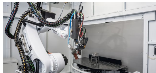
The laser network, serving a TruLaser 3030 fiber and a TruLaser Robot 5020, expands the range of services offered by SCS by adding laser cutting and welding.
