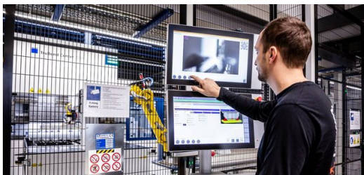
<p class="MAGAFIetext">The TecZone Bend programming software in combination with SimulEasy ensures process reliability. This allows 3D simulations including collision monitoring to be generated before the bending process.</p>
