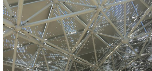
<p>For the SoFi, A. Zahner used three TRUMPF machines to cut and punch 37,000 different panels with around 30 million irregularly distributed holes. (Source: © A. ZAHNER COMPANY)</p>
