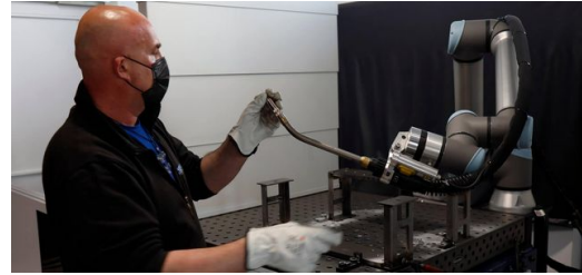
<p><span lang="EN-US">Even a lot size of 1 can be more profitable than with manual welding, because setting and especially "teaching" the robot arm is extremely simple. In the picture: Employee Blerim Limani at work on the TruArc Weld 1000.</span></p>
