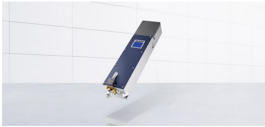
The TOP Cleave optics spread the power of an ultra-short pulse laser along the beam axis, creating a focus line. This increases by a hundred-fold the speed of separating glass using material modification, to one meter a second.
