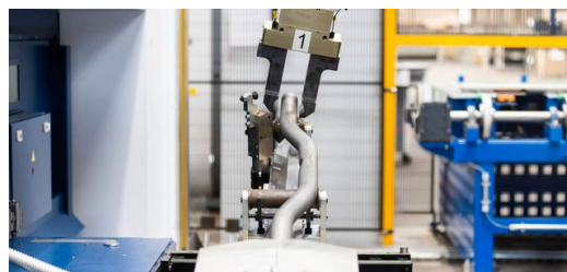
3D TruLaser Cell 8030 TRUMPF
